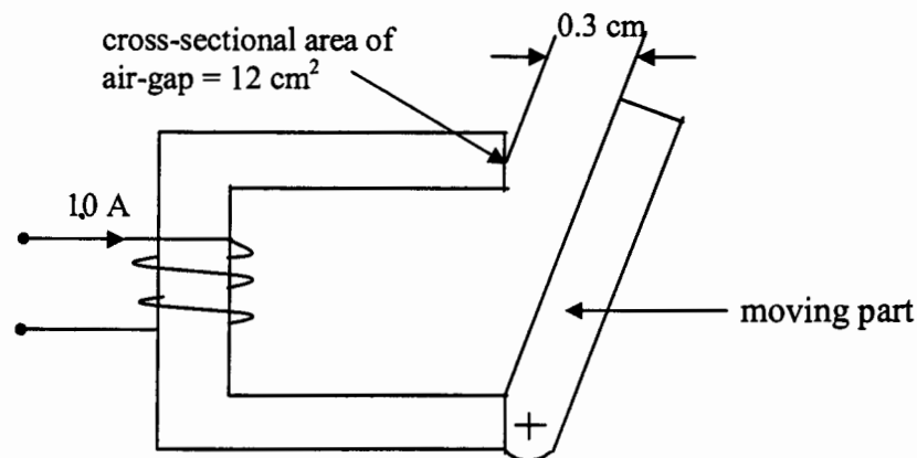
Fig. 1. Relay mechanism.
